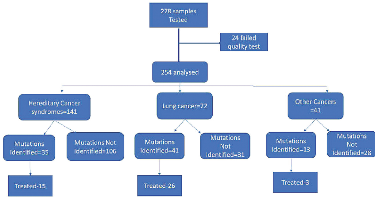
Fig. 1 Consort diagram.
